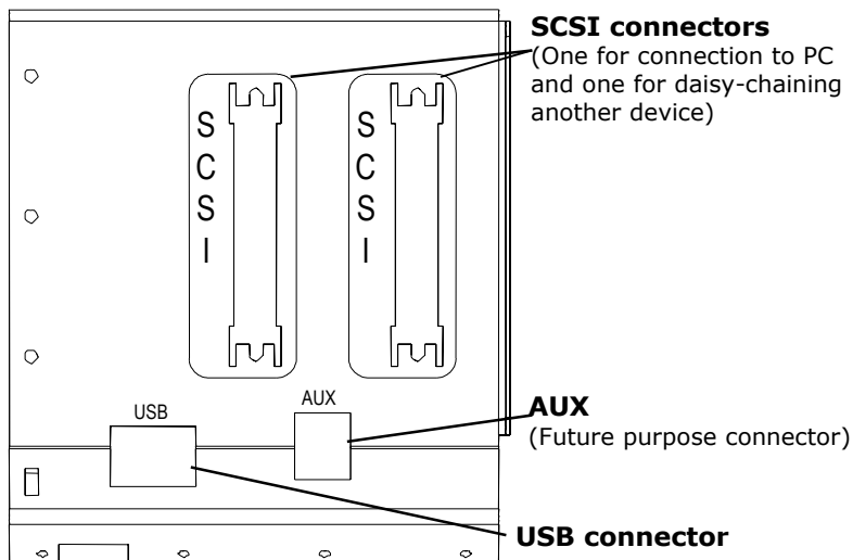
Figure 3-2 Scanner USB and SCSI Connectors on 25" & 36" Color Scanners
